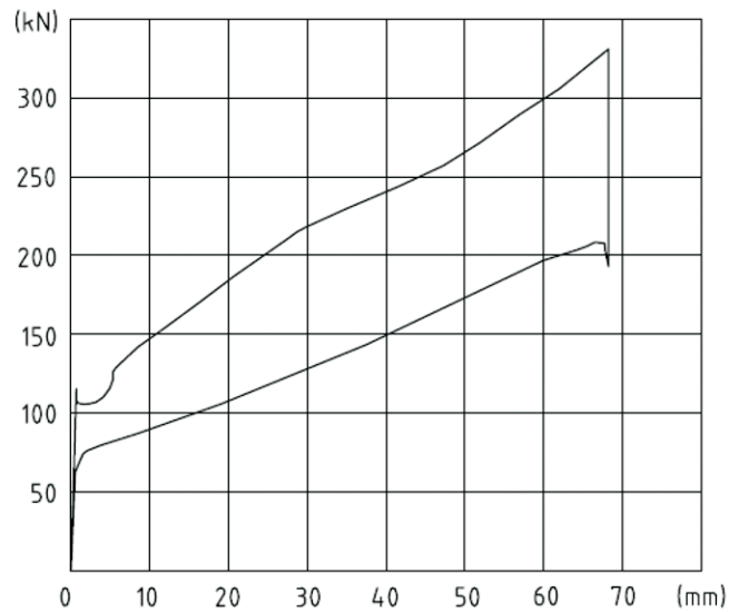
Static characteristic
