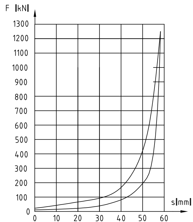
Static characteristic
